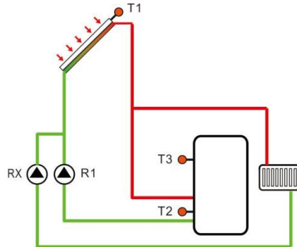
Heat transfer by collector pump logic
